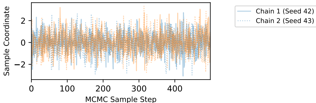
Chain Trajectory History ( u_{1,0} )
